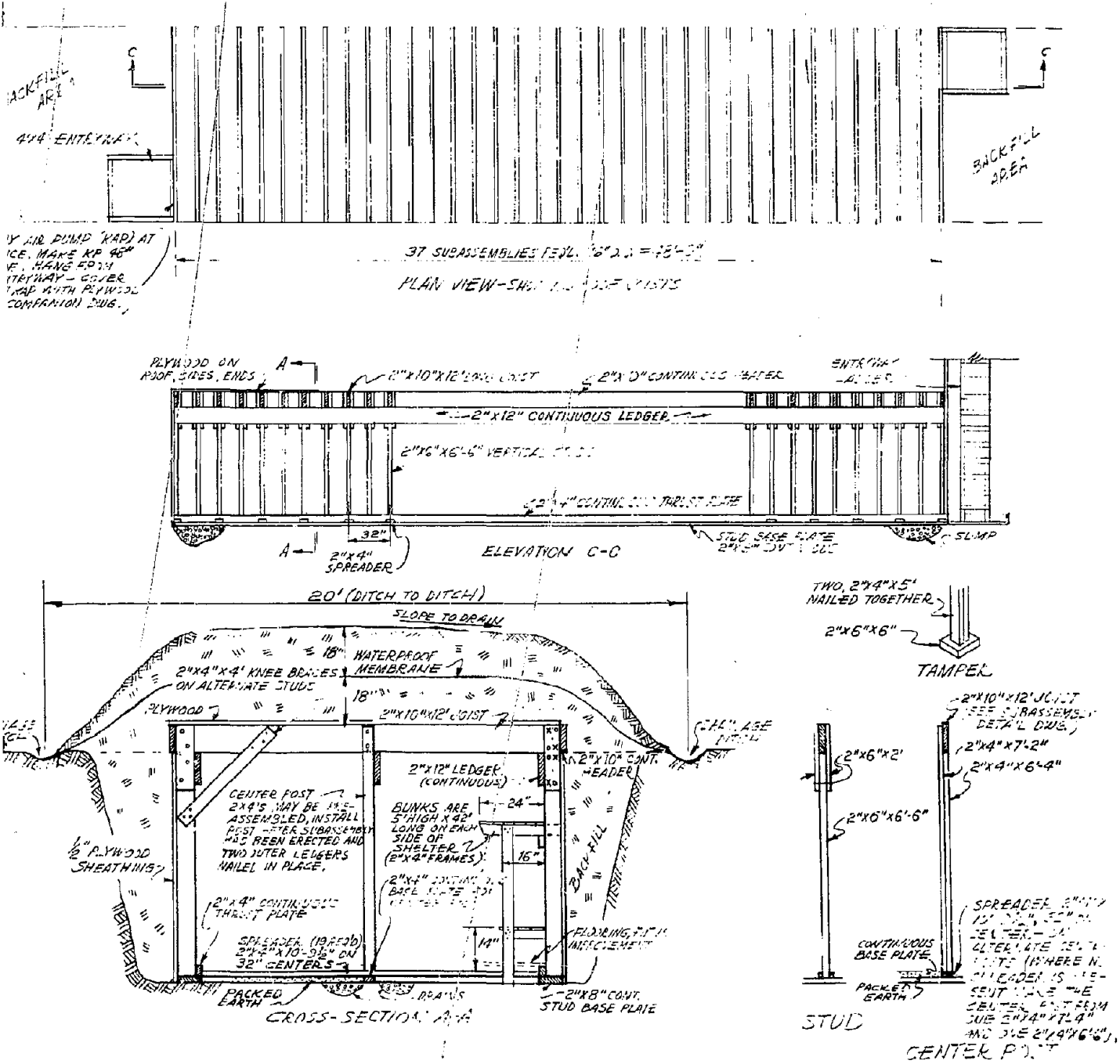
Fig. A-7.2. Rigid Frame Underground, Plan and Elevation.
